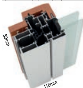
Sistema AM-B(rt) Système AM-B(rt) | AM-B(rt) System
