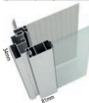
Sistema AM-B(rt) Système AM-B(rt) | AM-B(rt) System
