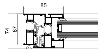
LT-Oculta | Concealed | Caché
