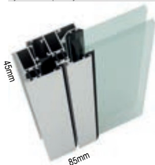
Sistema AT Système AT | AT System
