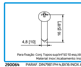
290064 PARAF. DIN7981 PH 4,8x16 INOX A2
