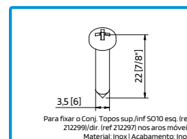
290031 PARAF. DIN7981 PH 3,5x22 INOX A2
